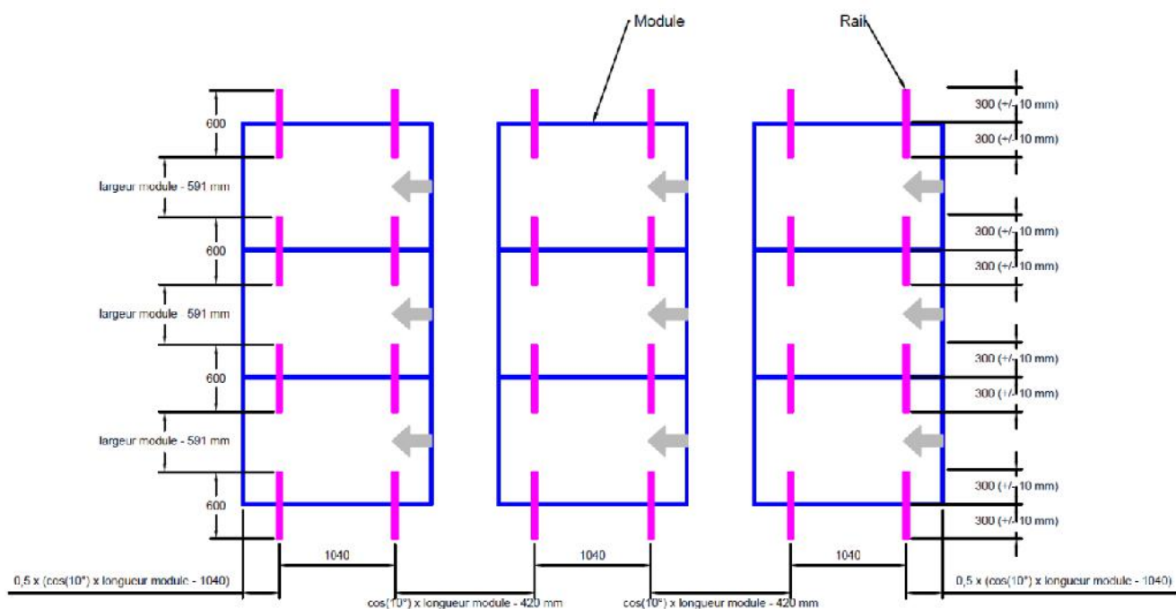
Figure 34 - Implantation des rails / modules simple shed
